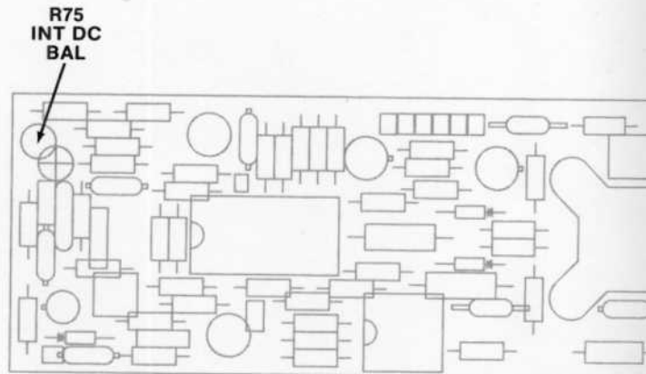
A8 MAIN TRIGGER
