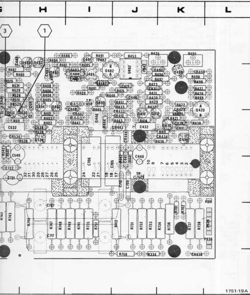
Board (SN B095740 & below).
