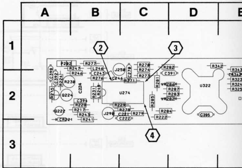
Fig. 8-11. A9-Delayed Trigger
