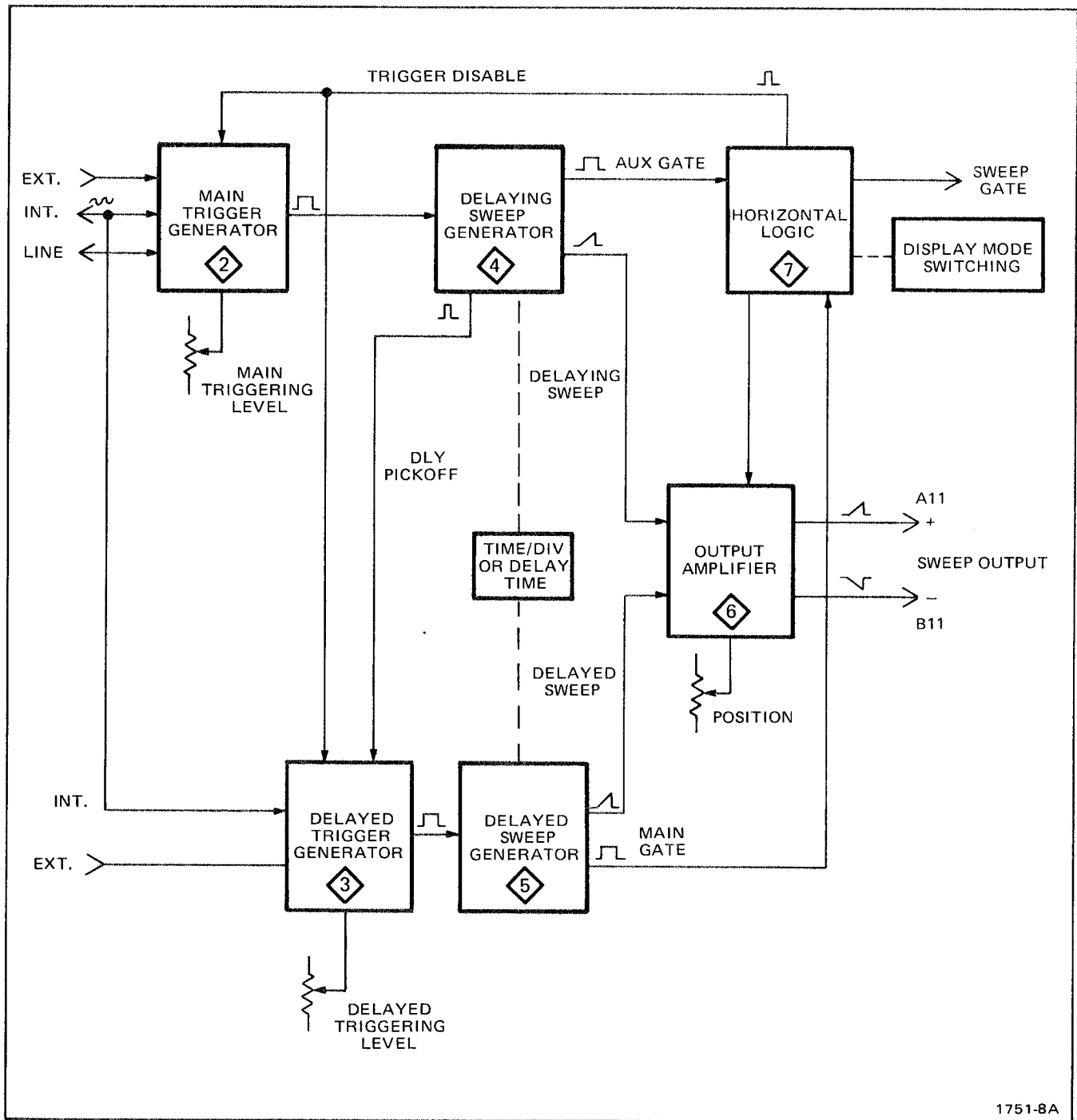
Fig. 8-2. Block Diagram.
