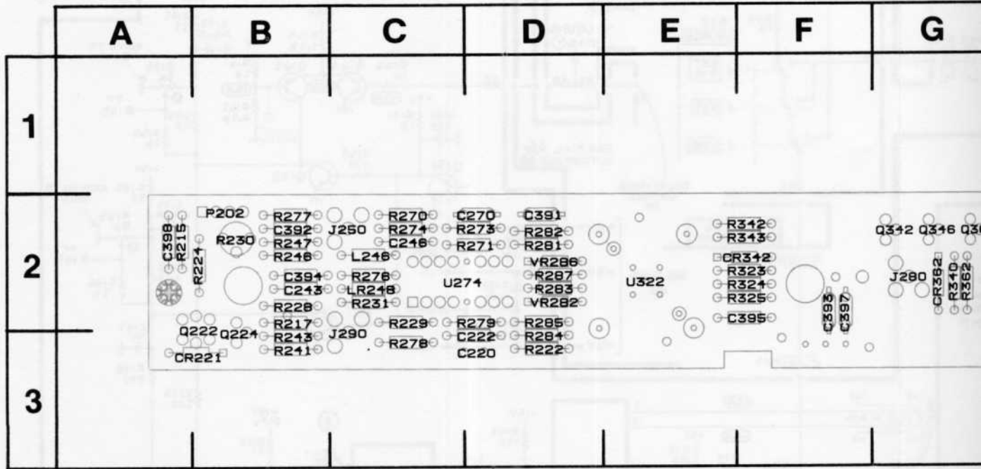
Fig. 8-10. A9-Delayed Trigger Circuit Board (SN
